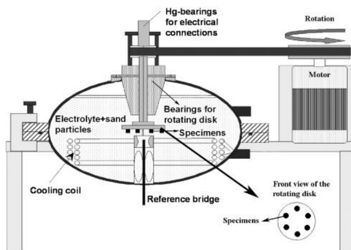
Figure 7. Scheme of the erosion–corrosion equipment, [30].
